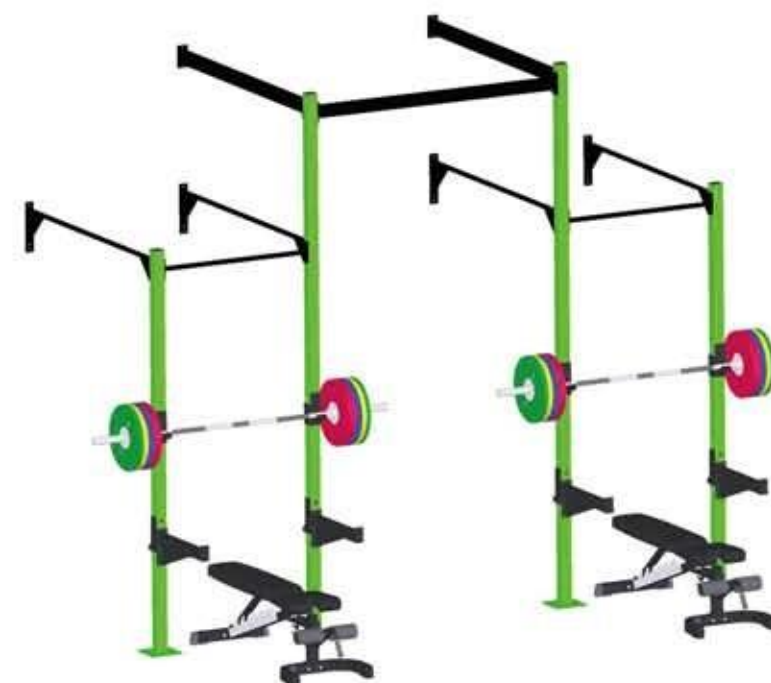
CF-006 Wall Mount Model Size:4'-6'-4'-4' Main tube:75*75*3mm,Monkey bar:Φ32*5mm Height:2.75m-3.6m,Depth:1.2m,Length:4.2m Color:Black matte/Green smooth
